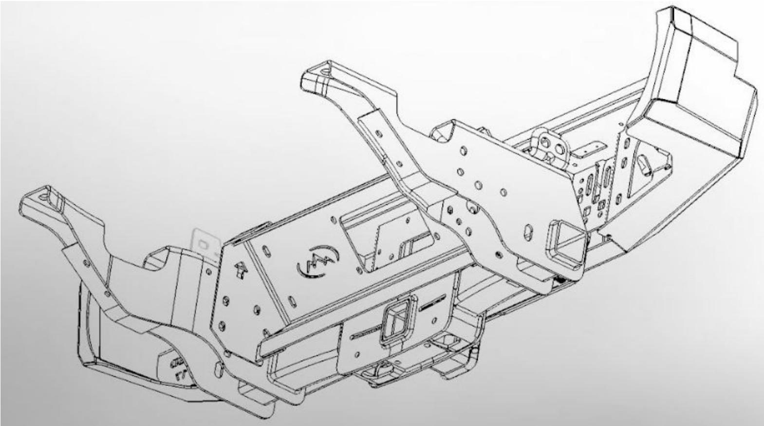
WINCH MOUNT CENTER SHOWN FOR REFERENCE
